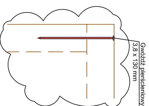
detail D
